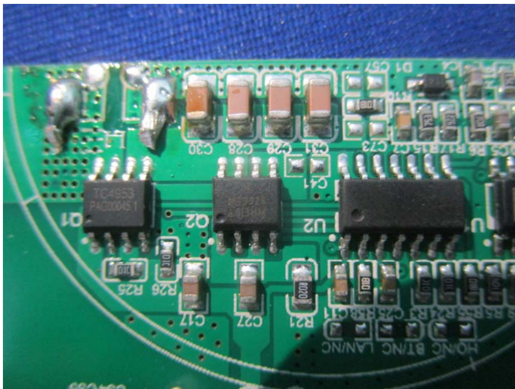
RF chip
