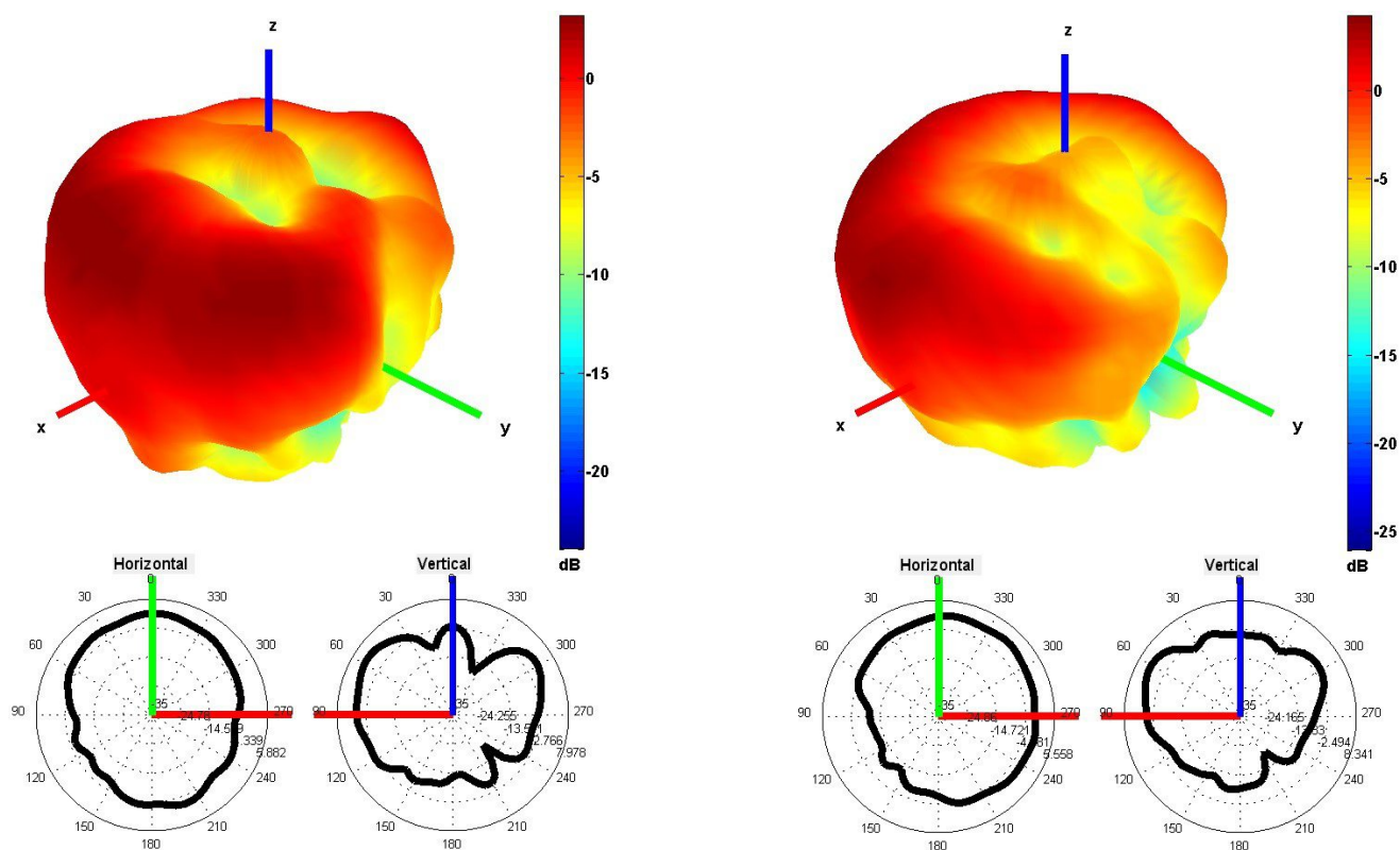
2100 and 2600 MHz Radiation pattern
