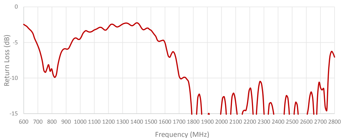
Cable 1: CELLULAR/LTE
