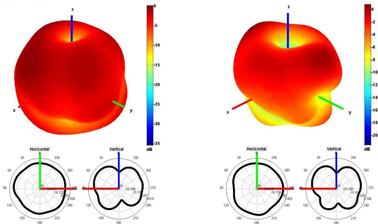
Cable 2: CELLULAR/LTE
