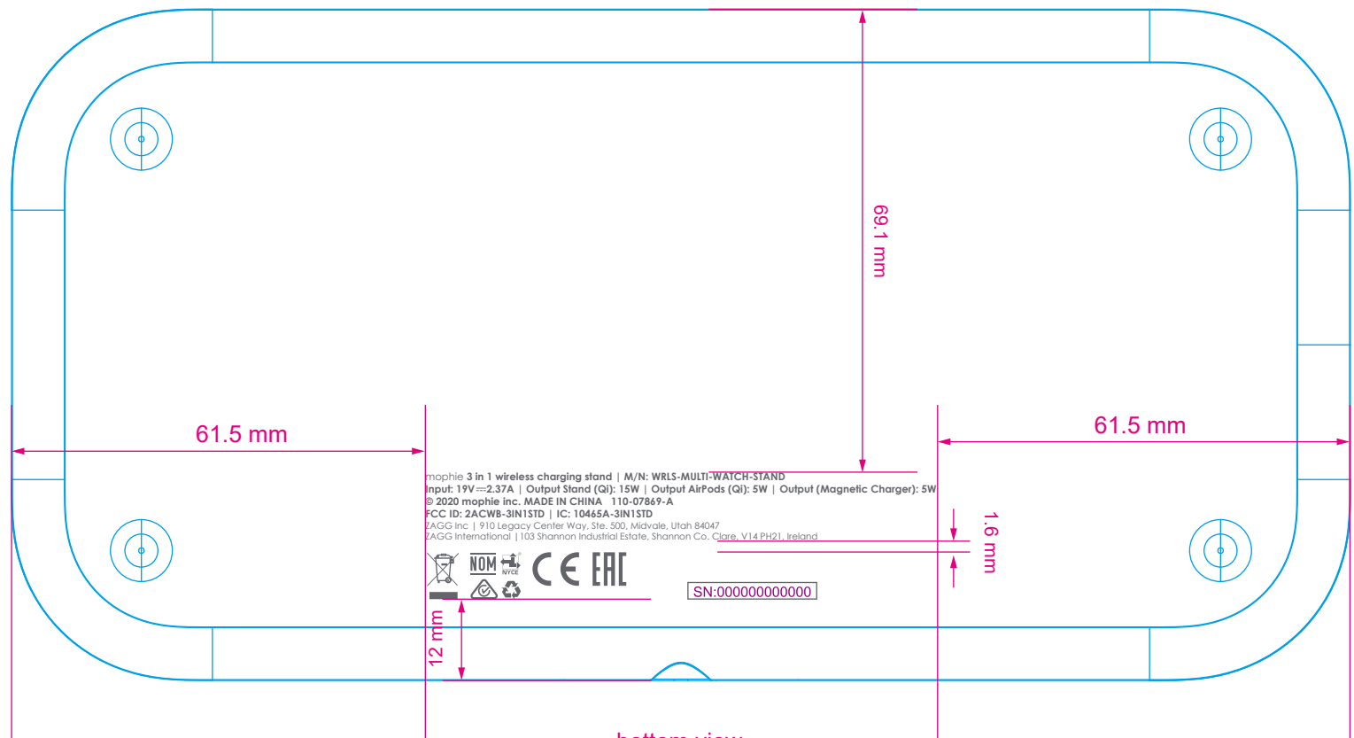
bottom view
