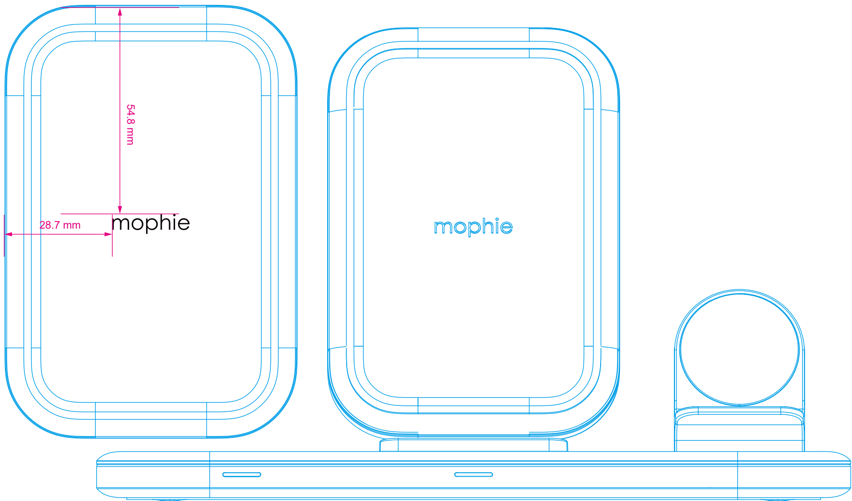
front view
