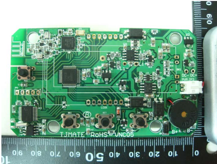
Front View of the EUT's PCB (Without LED panel)
