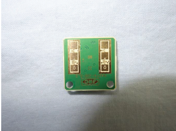
Antenna side
