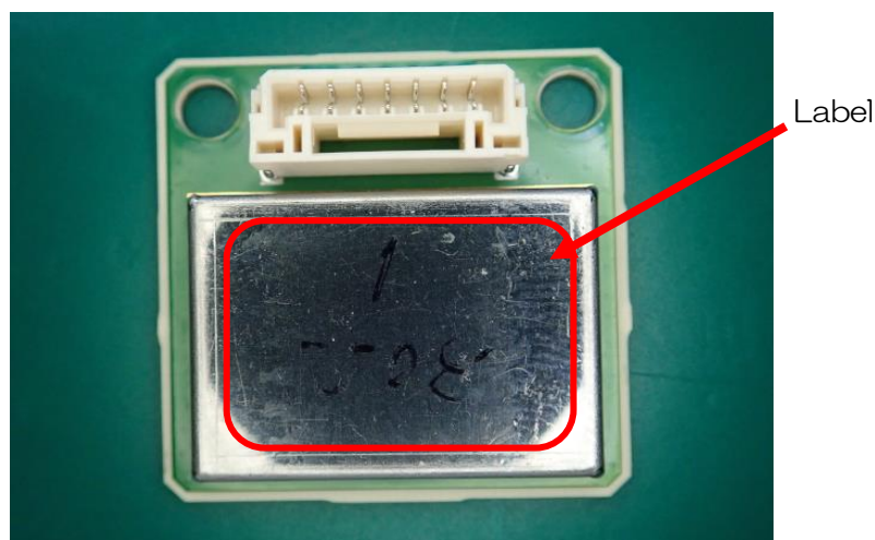
Back Side view: Metal Shielding Cover
