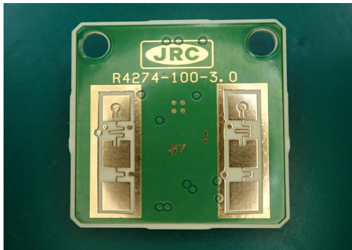
Front Side view: Patch Antenna
