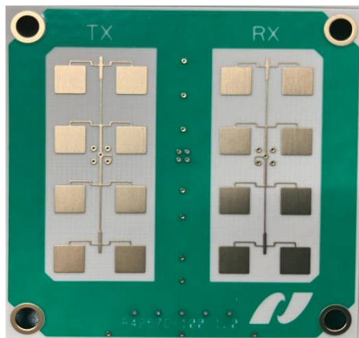
Front Side View: Patch Antenna
