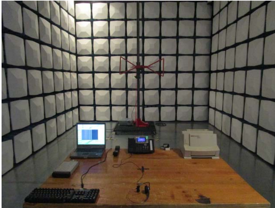
Radiated Emission -Front View (Below 1GHz) (Charging from Adapter)
