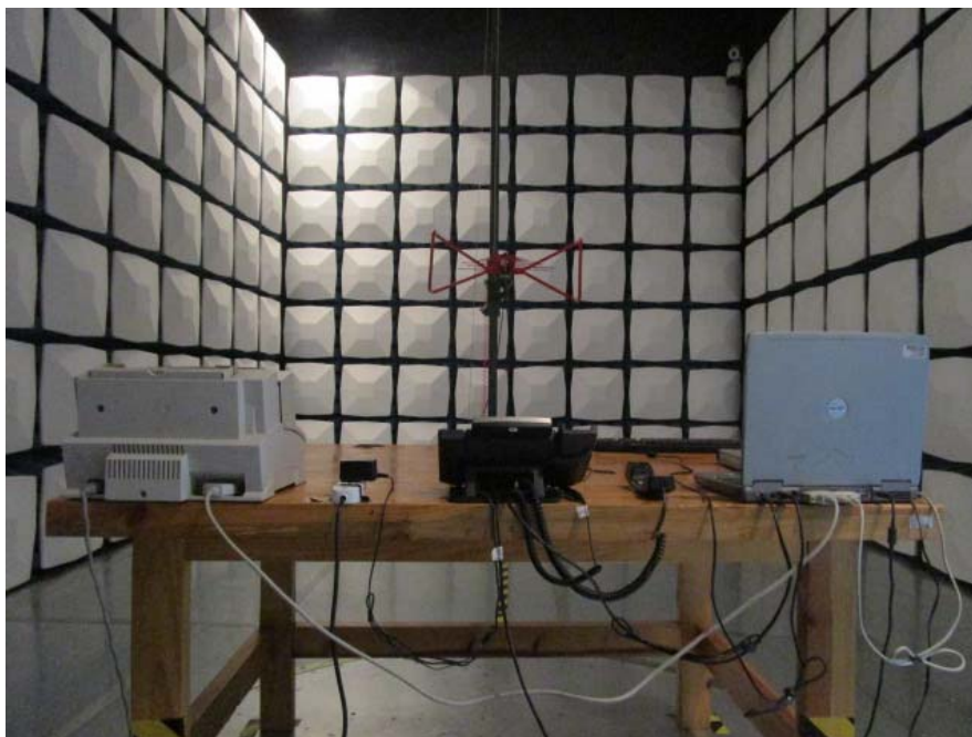
Radiated Emission - Rear View (Below 1GHz) (Charging from Adapter)
