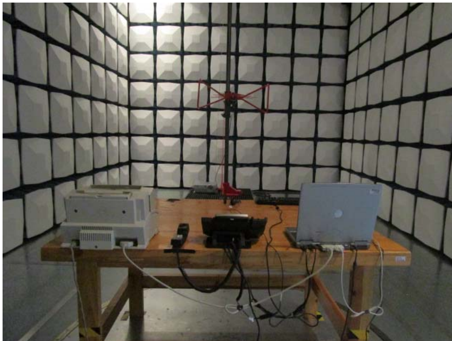
Radiated Emission - Rear View (Below 1GHz) (Charging from POE)
