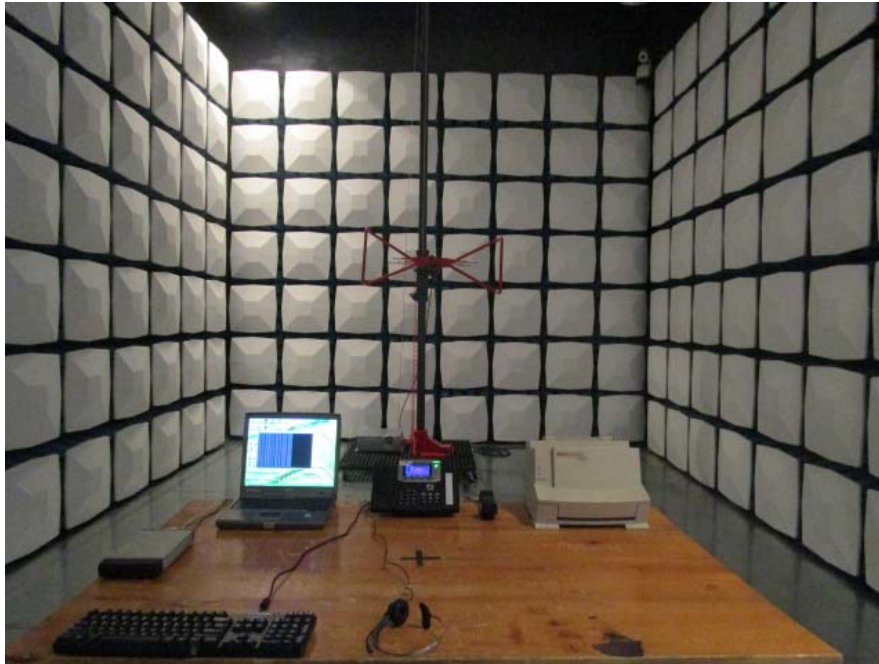
Radiated Emission -Front View (Below 1GHz) (Charging from POE)
