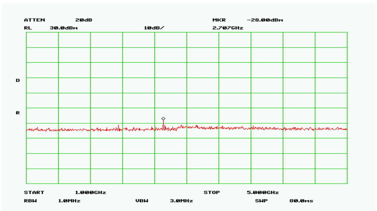
Plot 10 – Low Band – 1GHz to 5GHz
