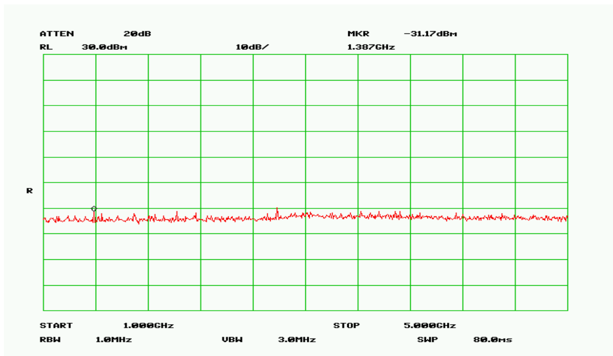
Plot 16 – High Band – 1GHz to 5GHz
