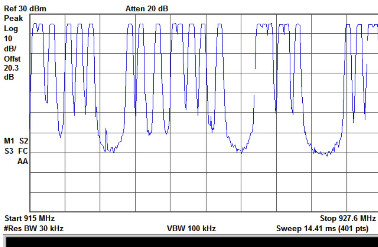
Plot 23 – Number of Frequency Hops – 915MHz to 927.6MHz
