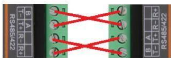
Figure 5. HF2211A RS422 Connection
