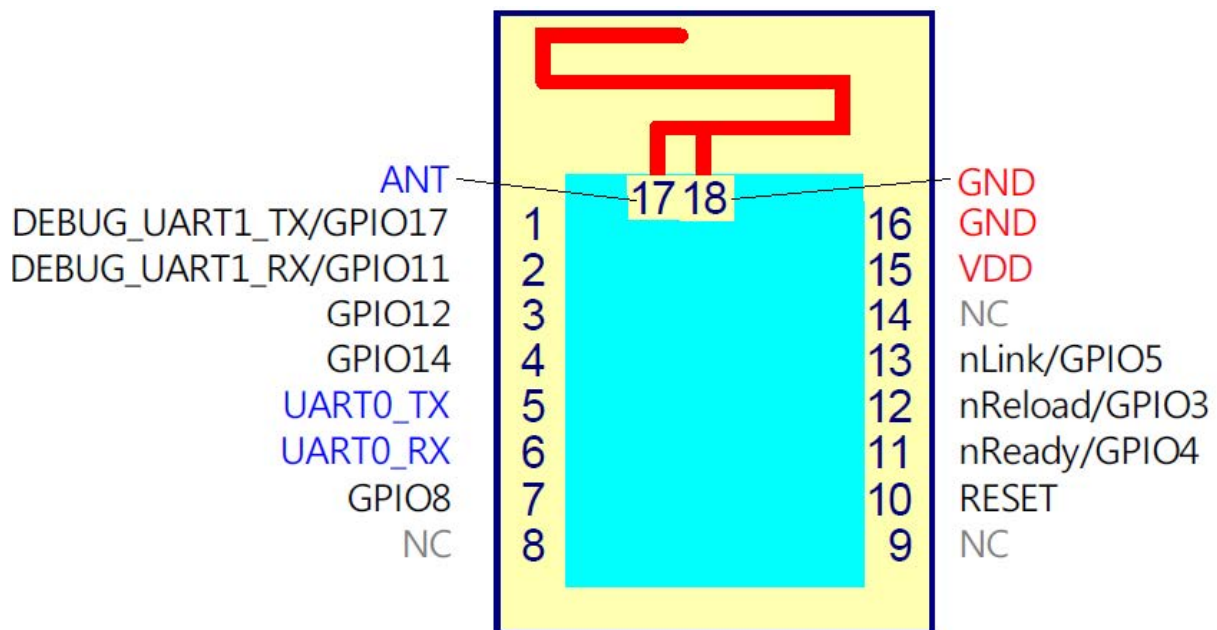
Figure 3. HF-LPT270 Pins Map
