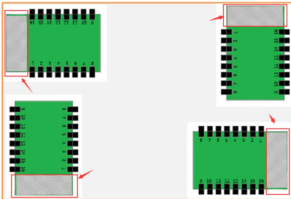
Figure 6. Suggested Module Placement Region
