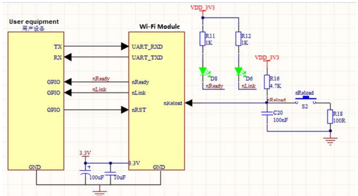
Figure 11. HF-LPT270 Hardware Typical Application
