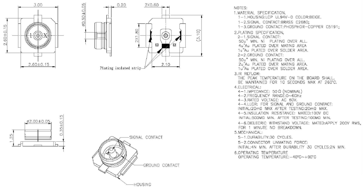
Figure 7. 1 st IPEX Connector
