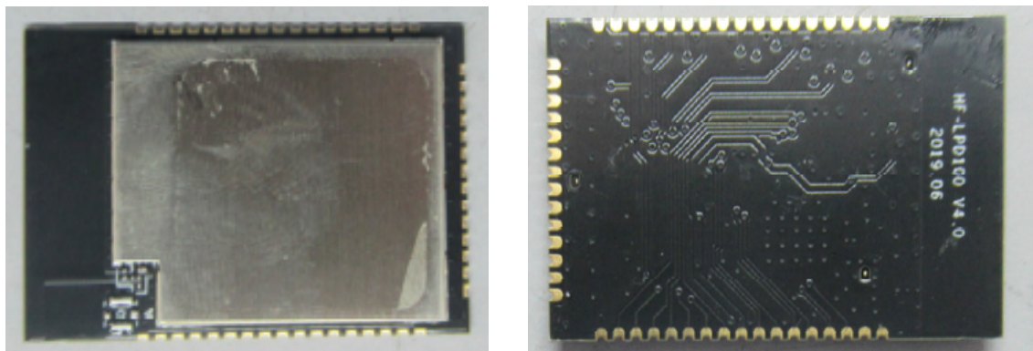
Figure 1. HF-LPD100 Appearance
