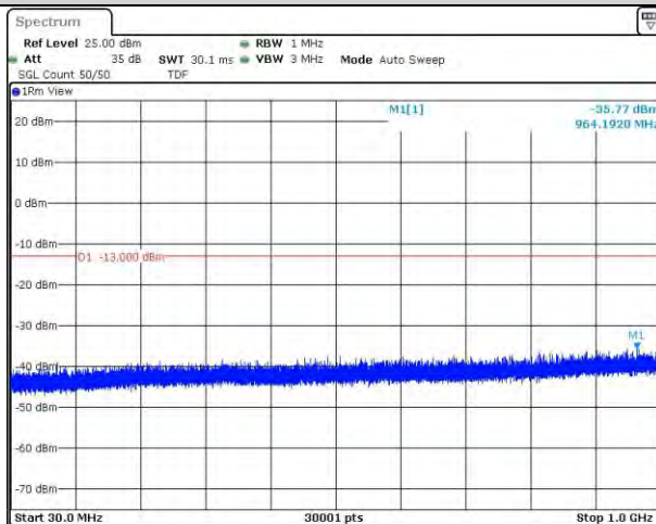
Band2-9262-30~1000MHz
