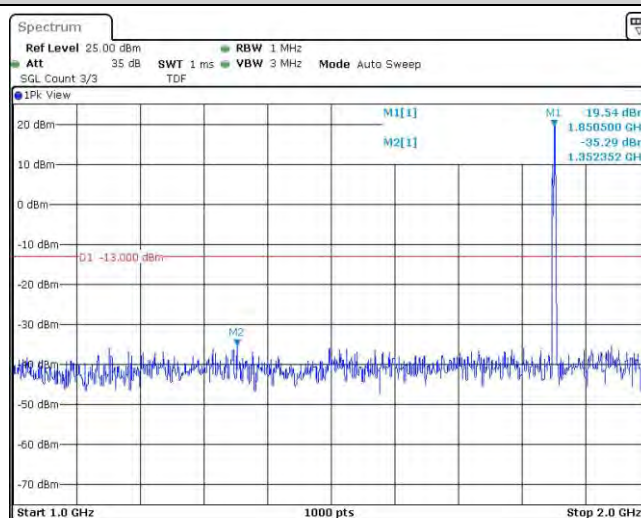
Band2-1.4MHz-QPSK-18607-1RB#0-Range2:1000~2000MHz
