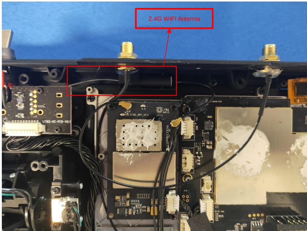
EUT UNCOVER VIEW (2.4G WIFI Antenna Close up photo)
