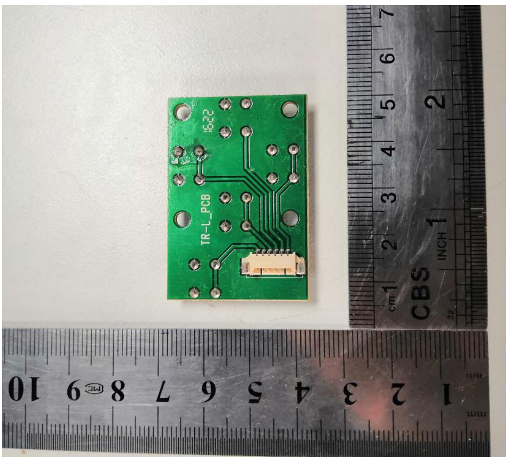
MAIN BOARD REAR VIEW
