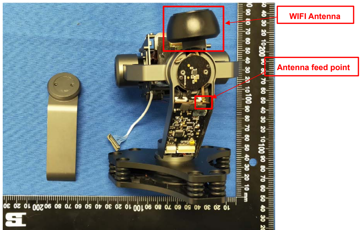
EUT UNCOVER VIEW 3
