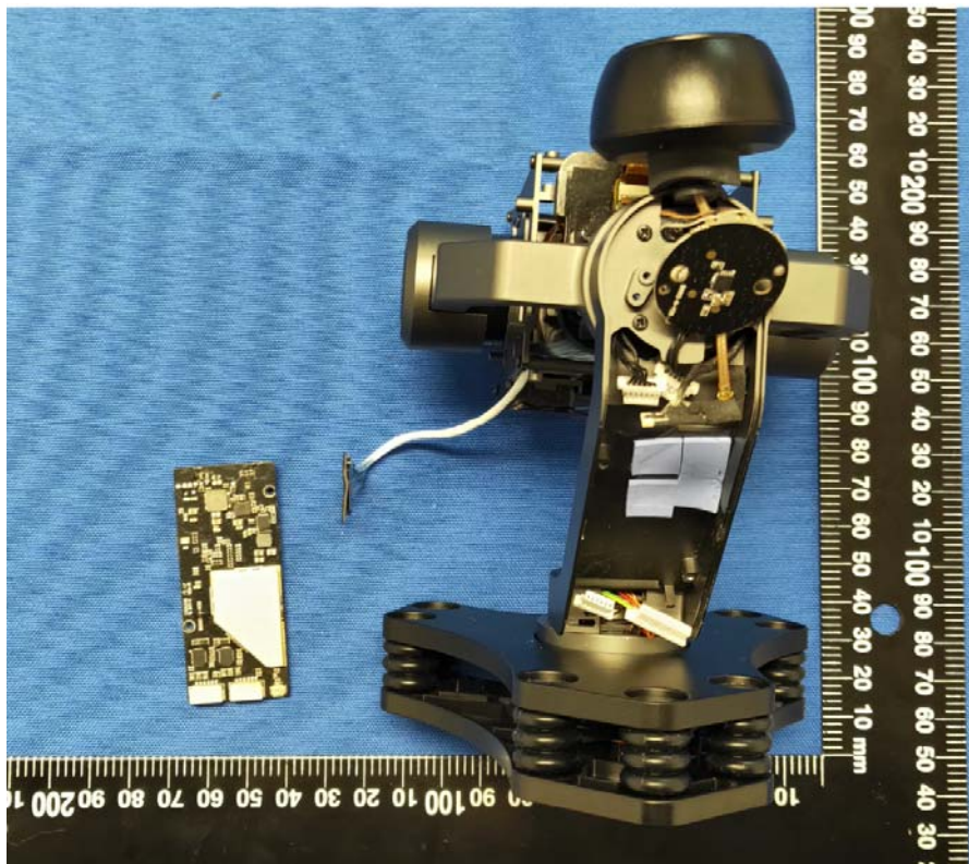
EUT UNCOVER VIEW 4
