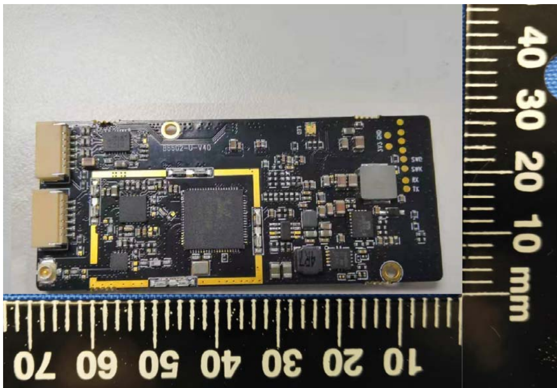
MAIN BOARD REAR VIEW
