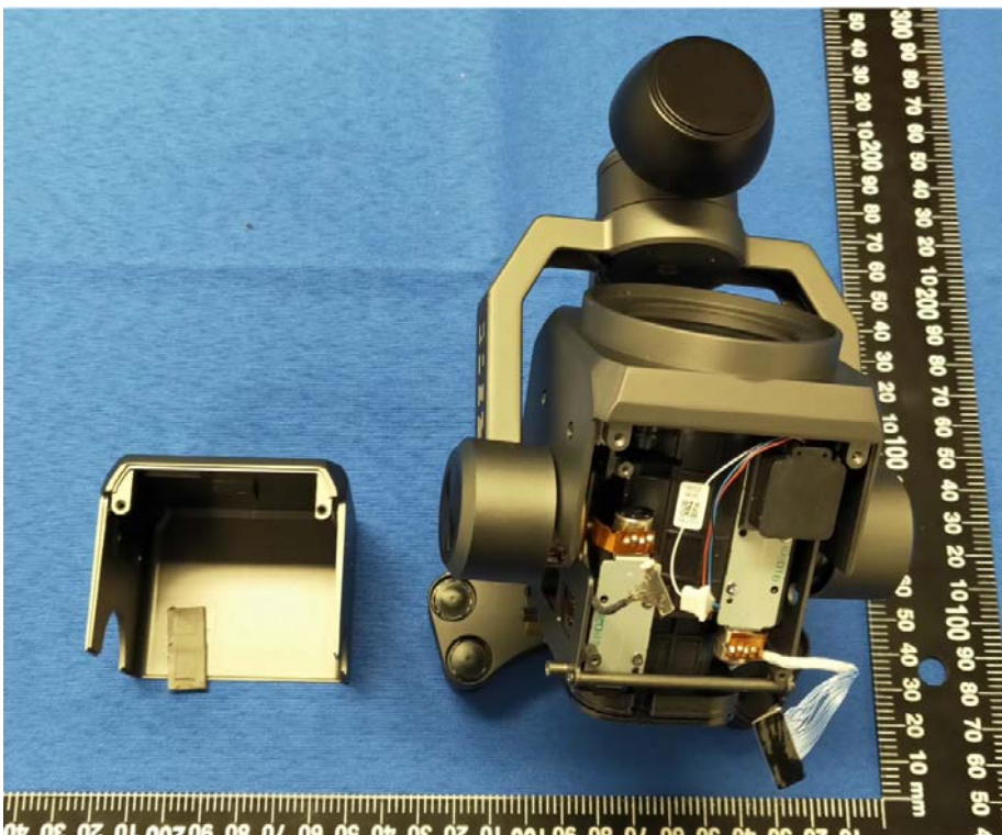
EUT UNCOVER VIEW 2
