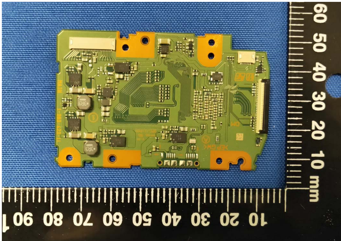
MAIN BOARD REAR VIEW
