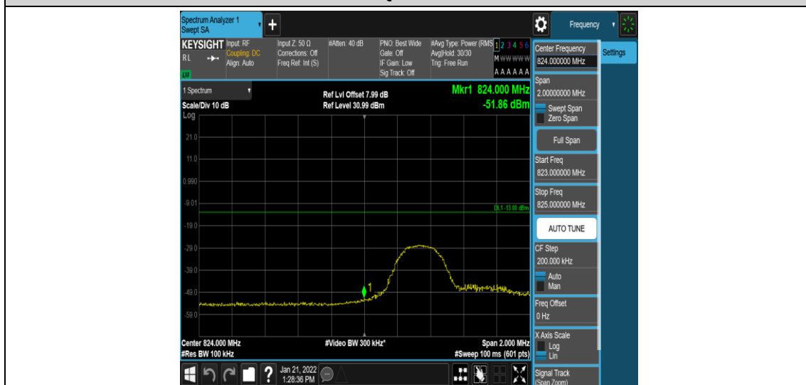
Band5-5MHz-QPSK-20425-1RB#24
