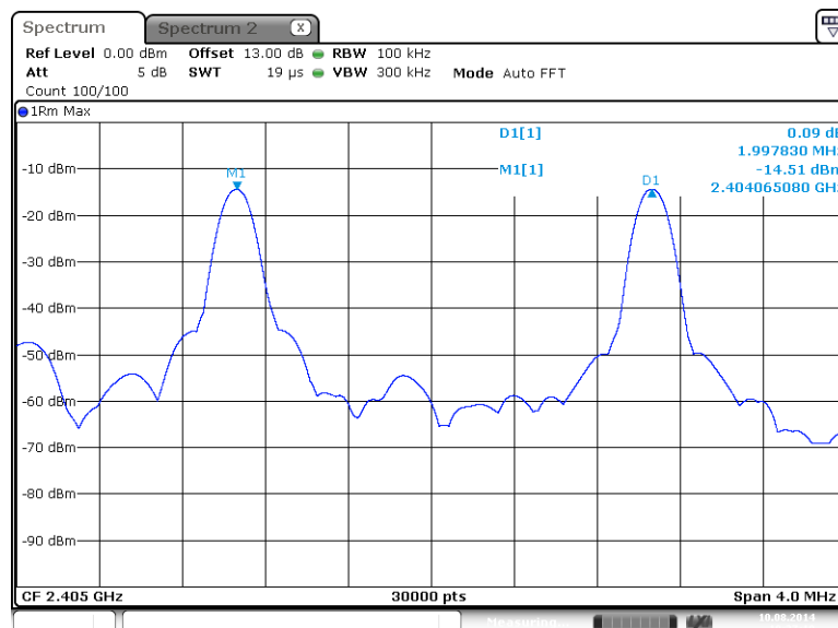
Plot 7.2.2 Carrier frequency separation
