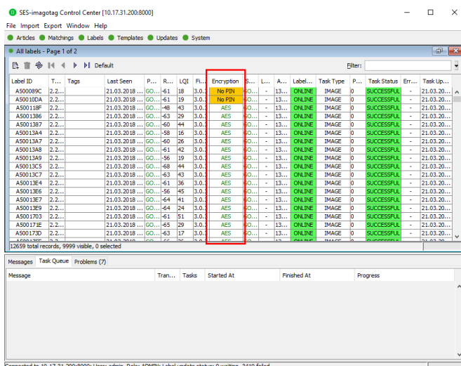
FIGURE 1-24: Encryption status
