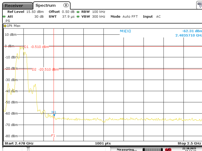
No-hopping mode
