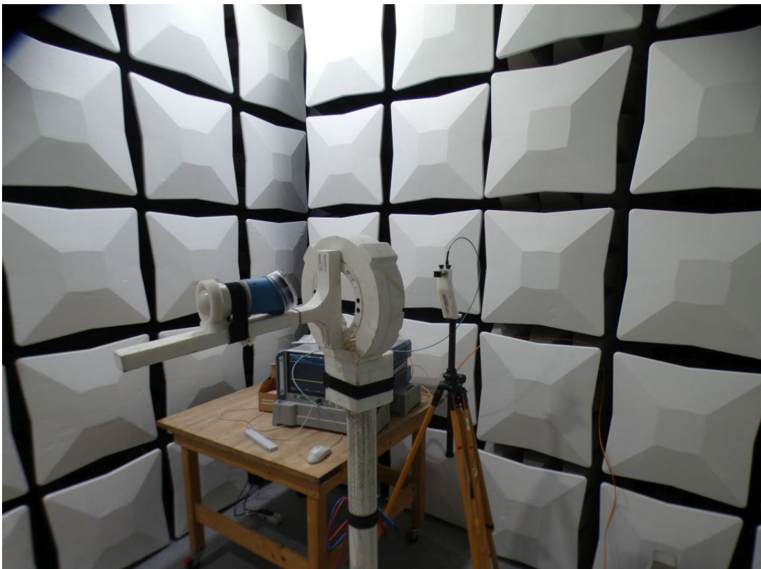
Photo 6: Test setup for radiated measurements above 26 GHz
