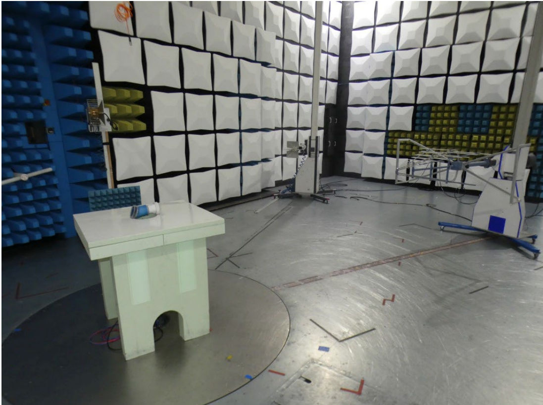
Photo 3: Test setup for radiated measurements below 1 GHz
