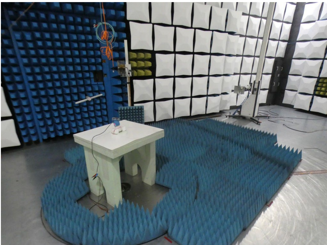
Photo 4: Test setup for radiated measurements above 1 GHz
