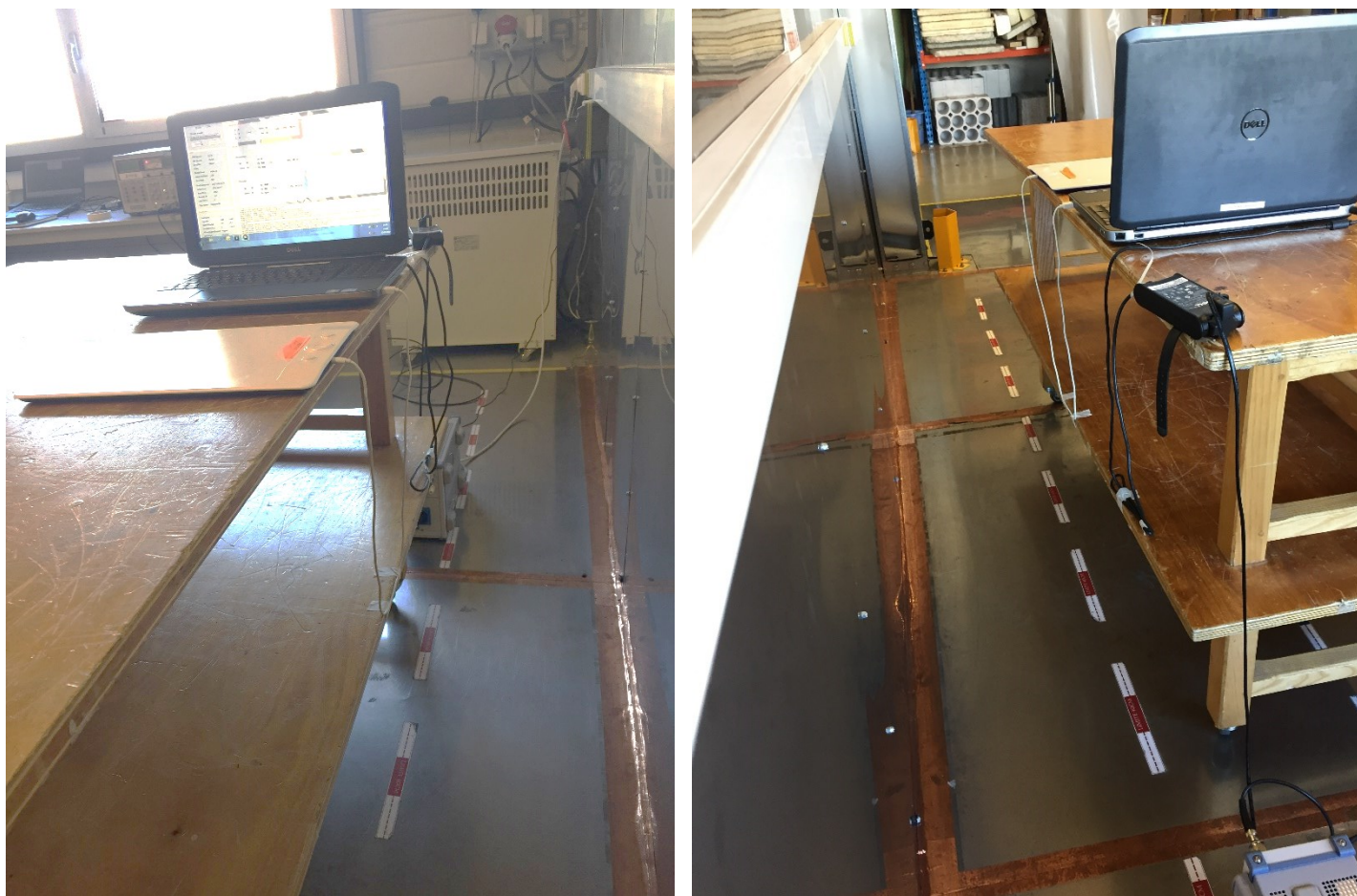
Test setup
