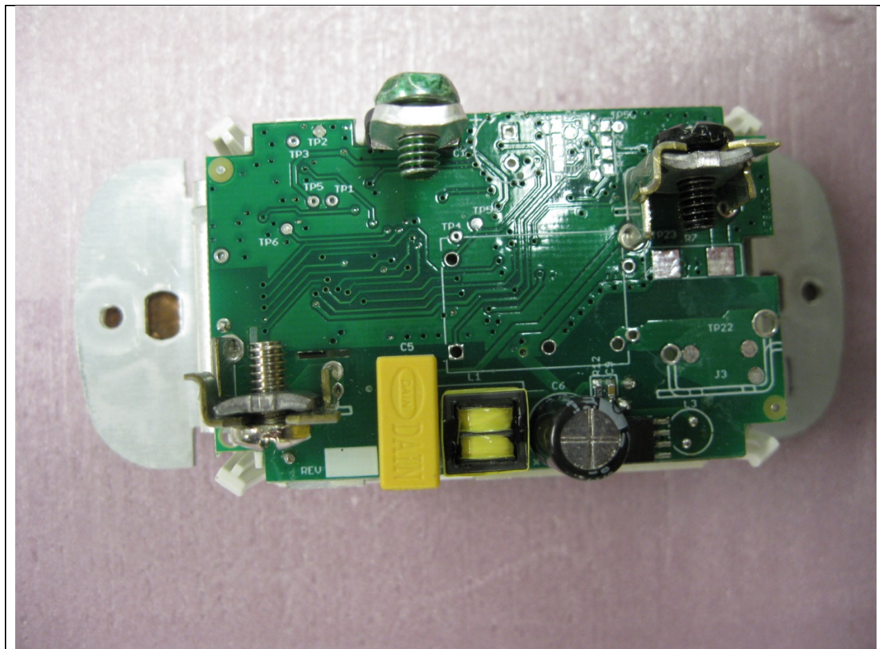
Bottom Side of Switch/Dimmer Board (Power)
