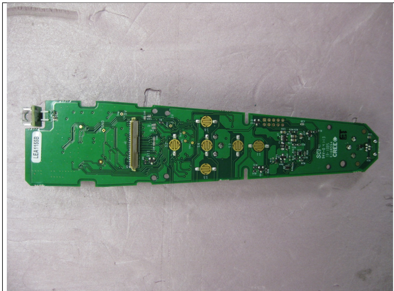
Commissioning Tool – Top of PC Board (Display Removed)
