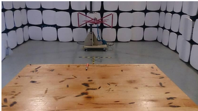
Radiated Emission(30MHz-1GHz)
