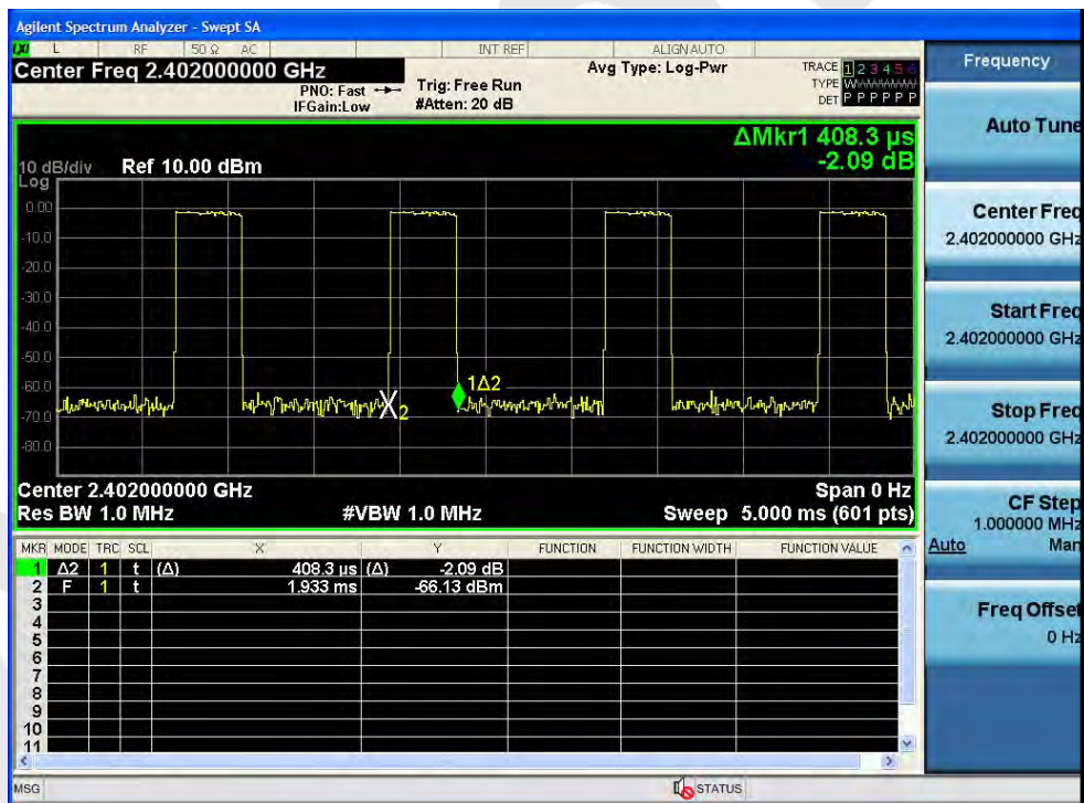
Test Mode: EDR---3DH1
