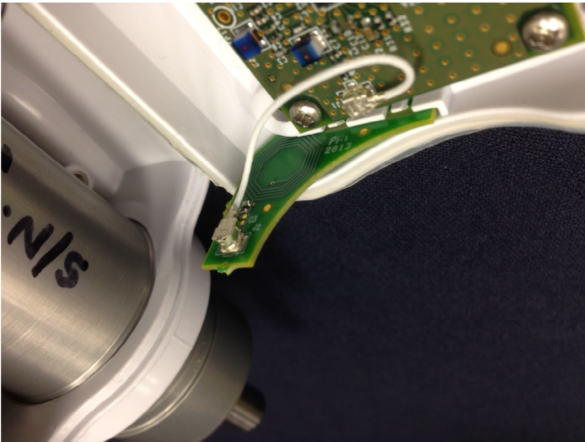
Figure 3: RF Board Mounted to TW Top Enclosure
