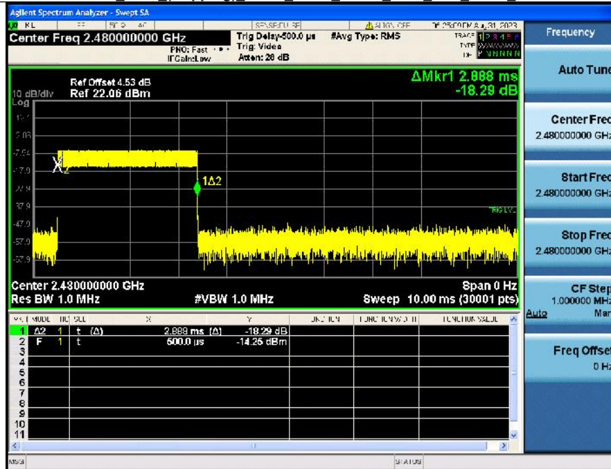
Dwell_Time_(Hopping)_NVNT_ANT1_1-DH5_2480_Accumulated
