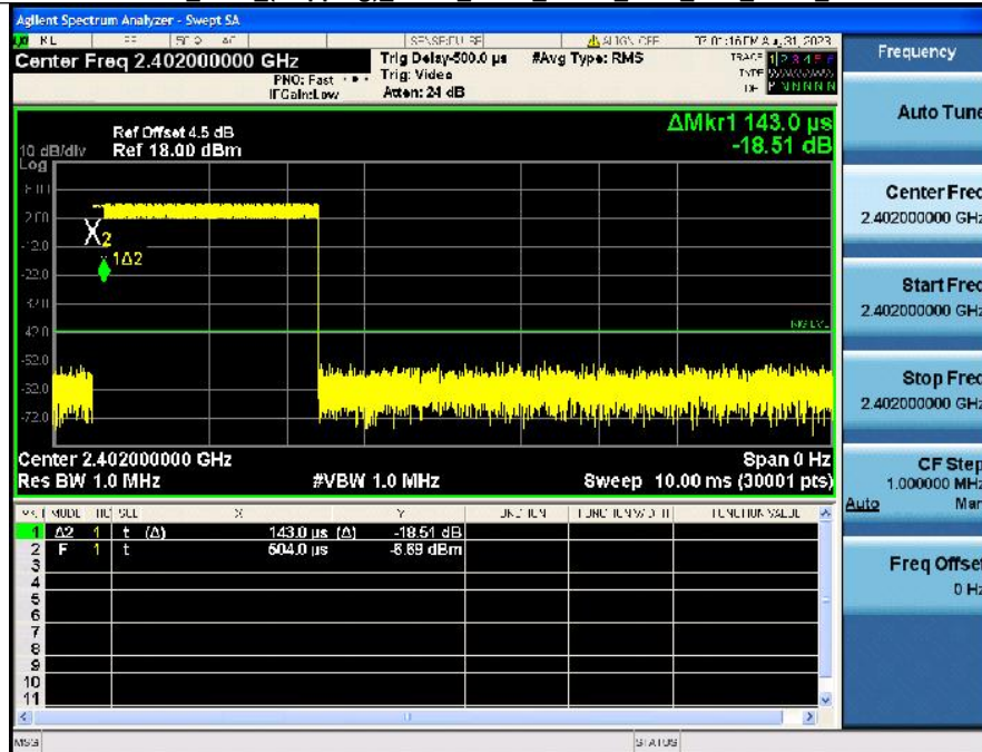
Dwell Time (Hopping) NVNT_ANT1_2-DH5_2402_Accumulated
