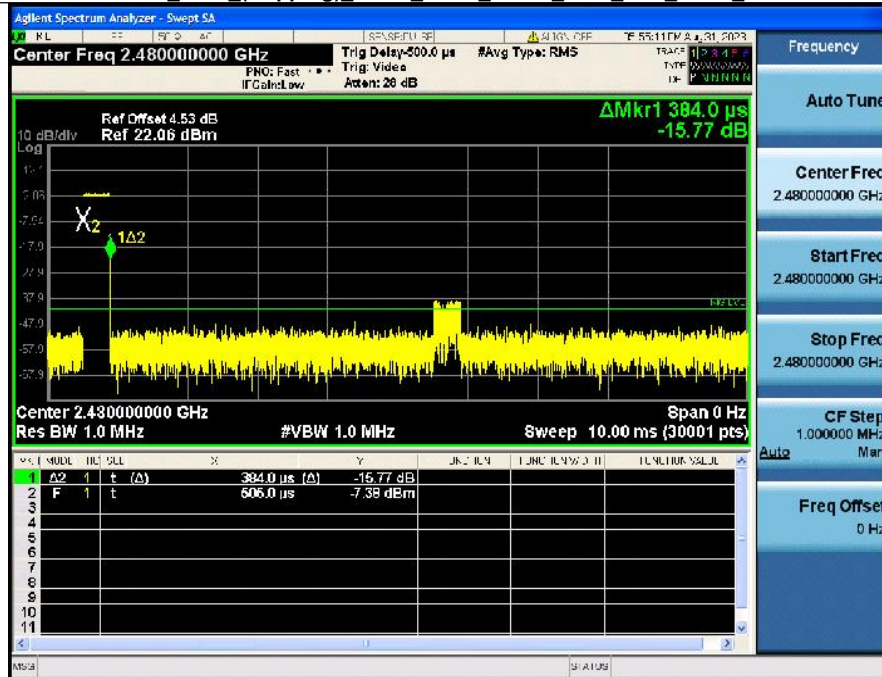
Dwell Time (Hopping) NVNT_ANT1_1-DH1_2480_Accumulated
