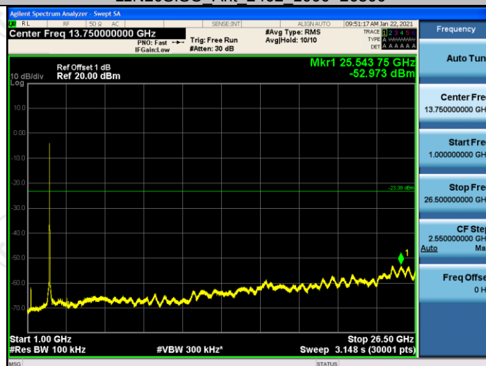
11N40SISO Ant 2422 0~Reference
