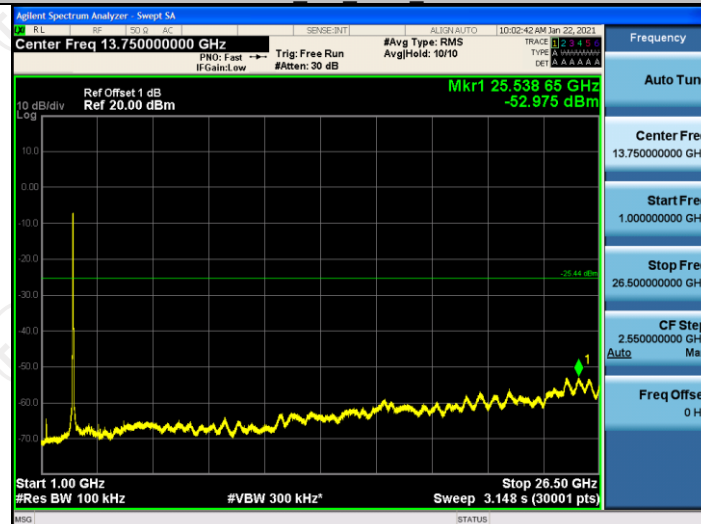
11N40SISO Ant 2452 1000~26500
