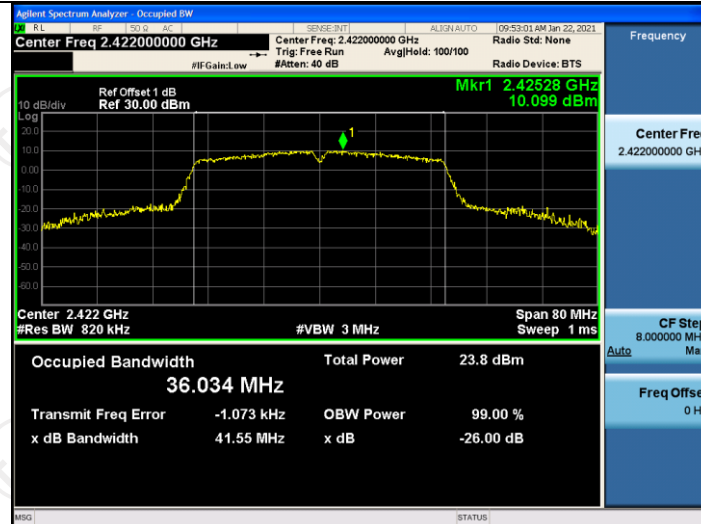
11N40SISO Ant 2437
