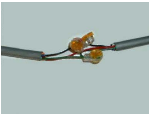
A correct wire splicing using UY gel cap connectors. A correct insertion of the splice in the burial pod.
