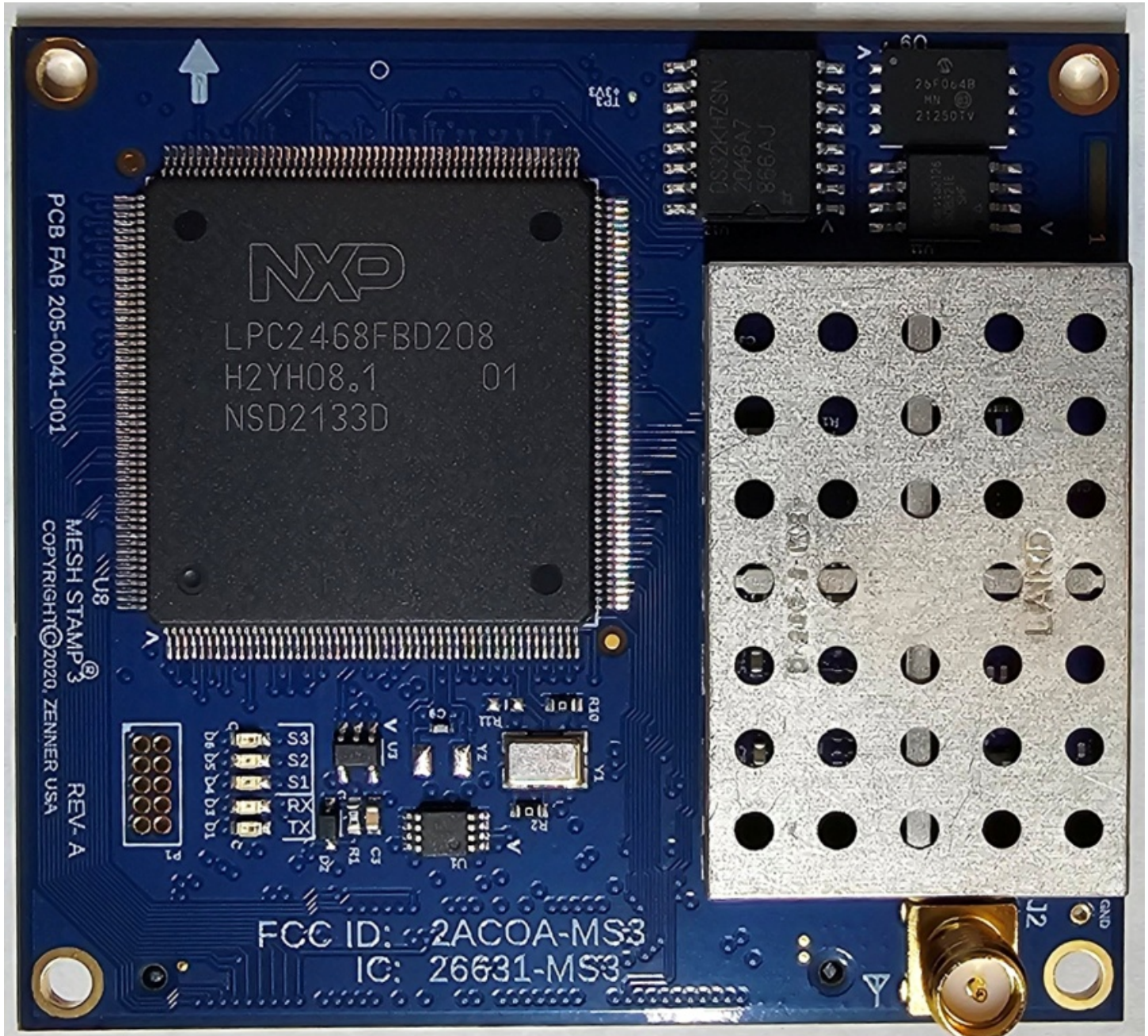
Figure E16.1 – External, Top
