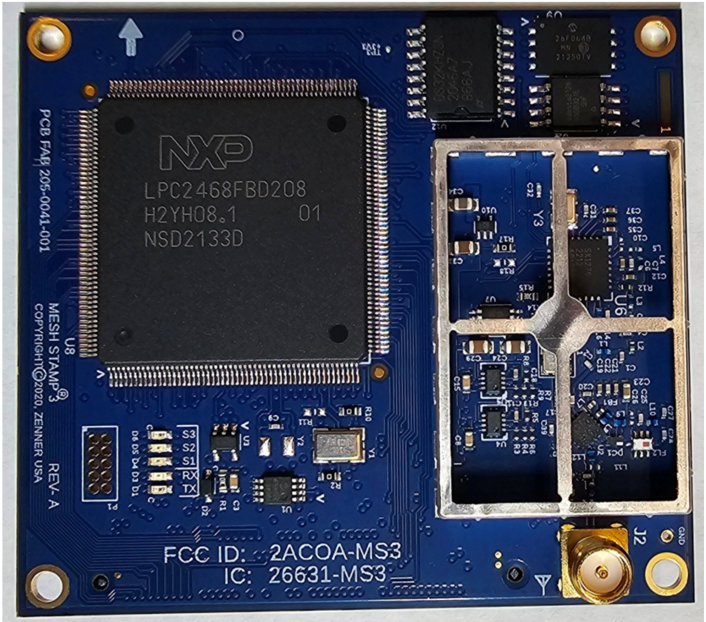
Figure E16.2 – External, Top, Shield Removed
