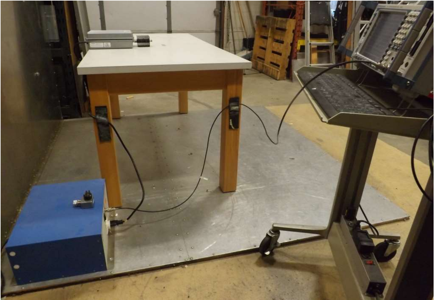
Figure E18.5 – Setup, Line Conducted Emissions
