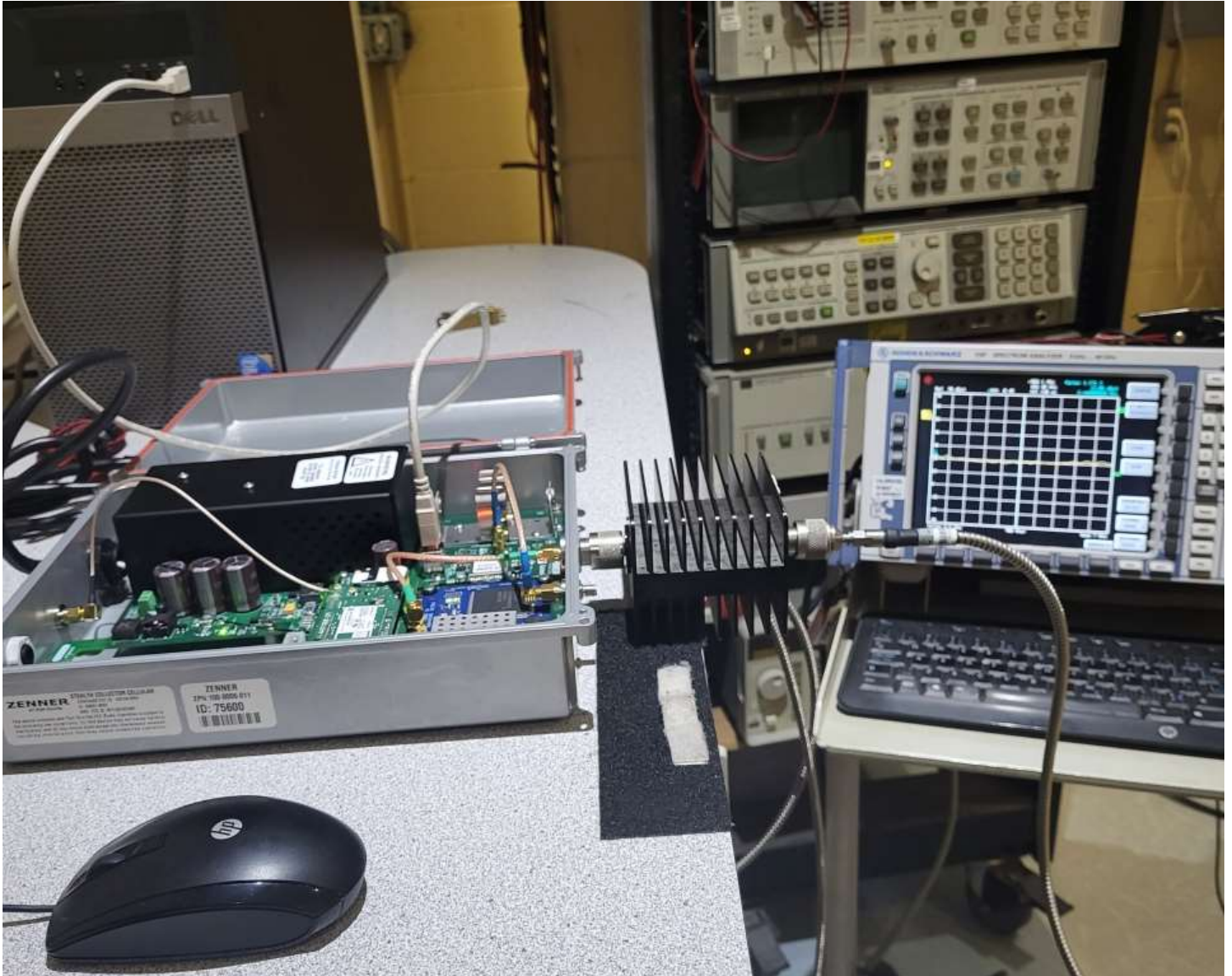
Figure E18.1 – Setup, Antenna Port Conducted
