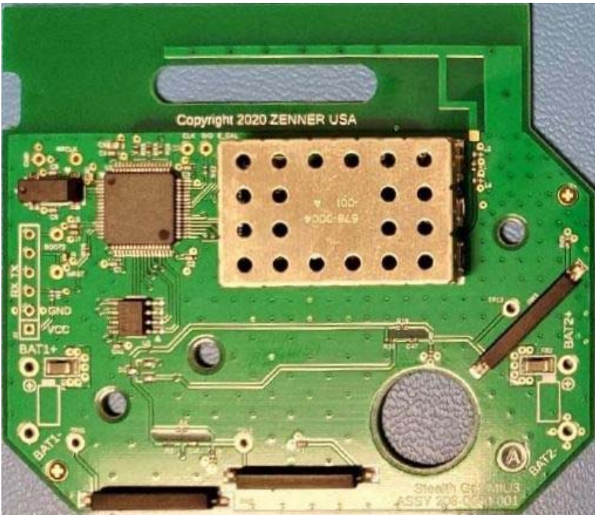
Figure E22.2 – PCB Top
