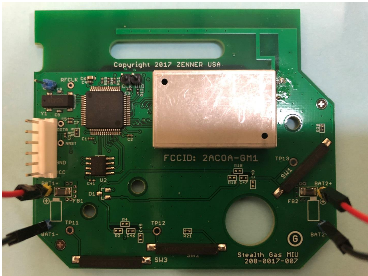
Battery Connected
