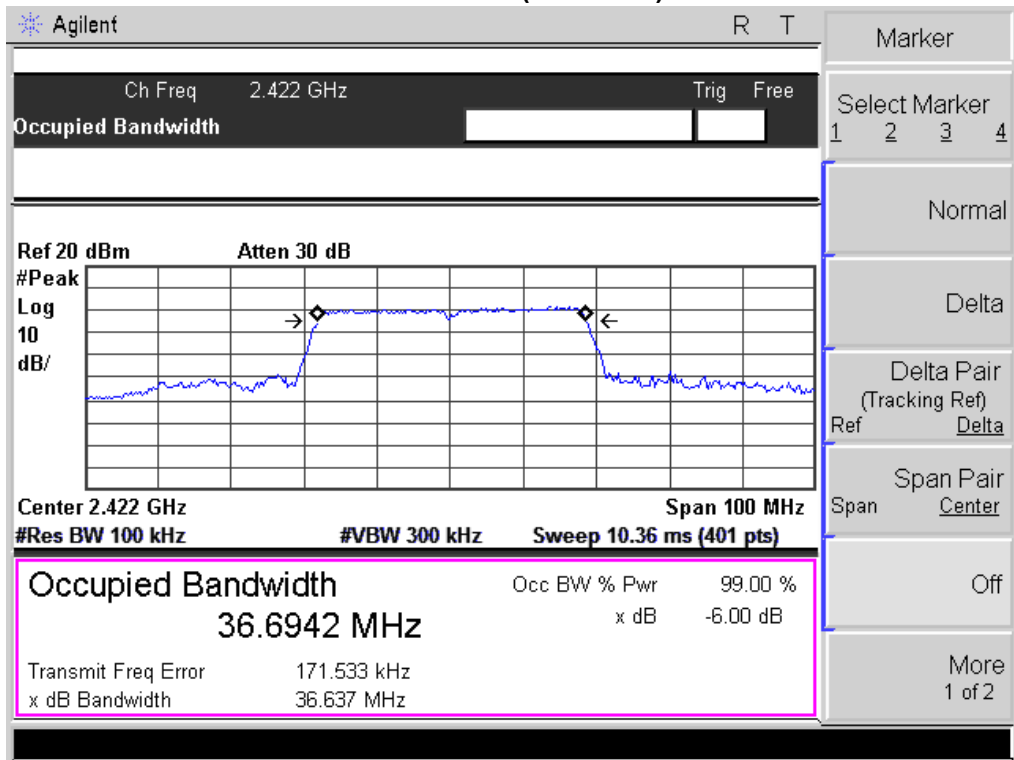
Channel 03 (2422MHz)
