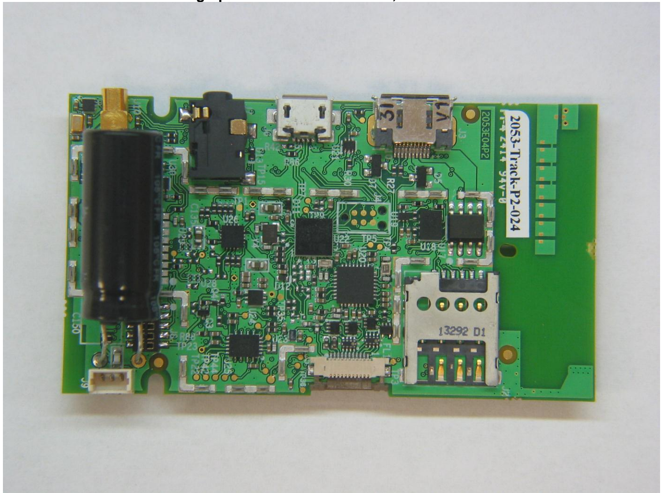
Photograph of PC Board: Foil Side, Shield removed
