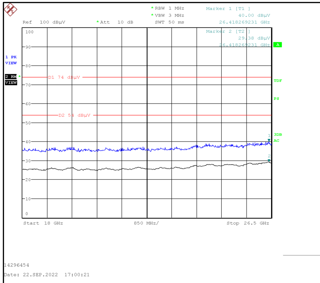
Plot: 18 GHz – 26 GHz: BT-LE / 2 Mbps / PRBS9 / PWR 0 dBm / Top Channel / PCB Antenna
