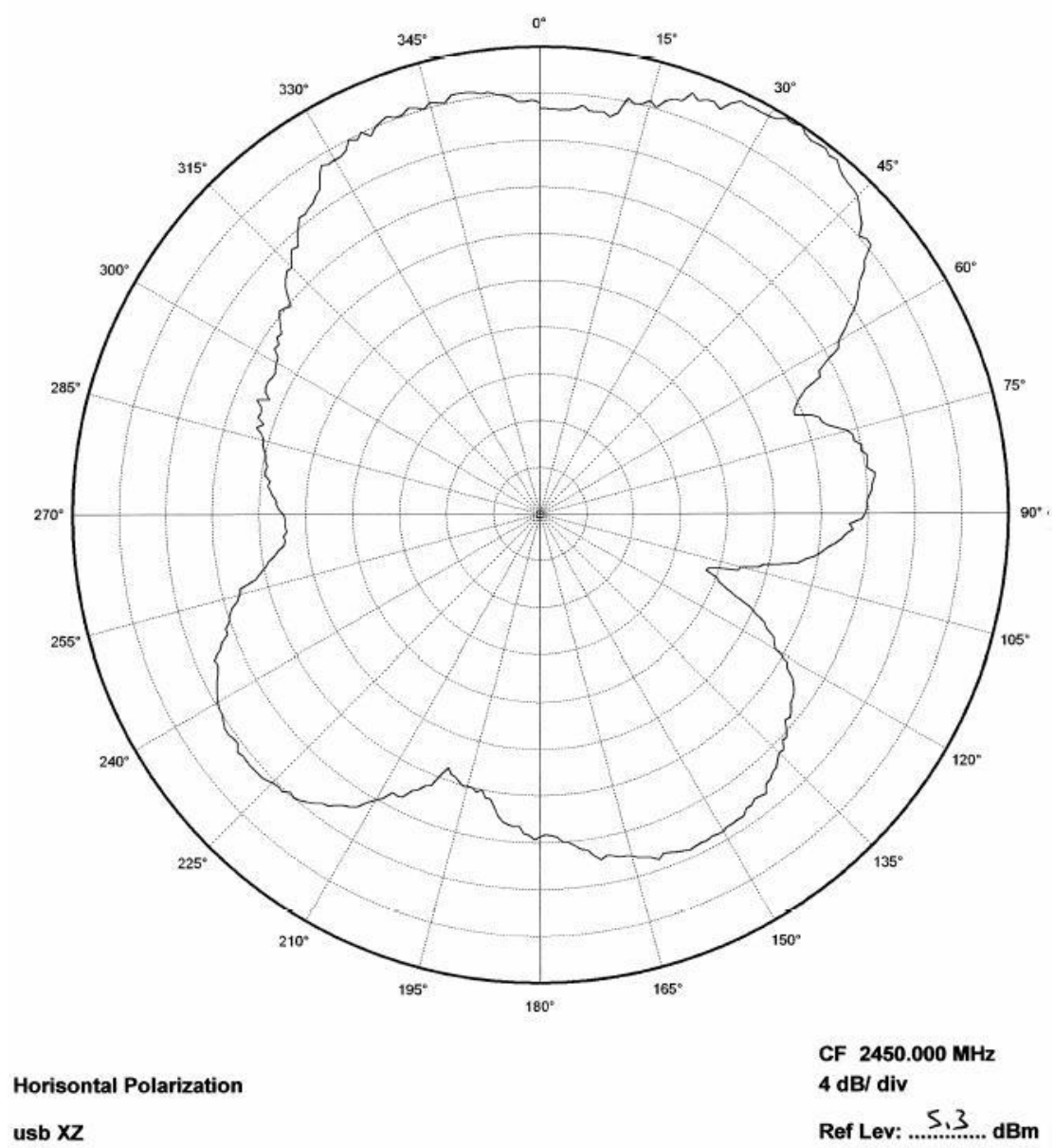
Figure 10: D63Beacon XZ Plane
