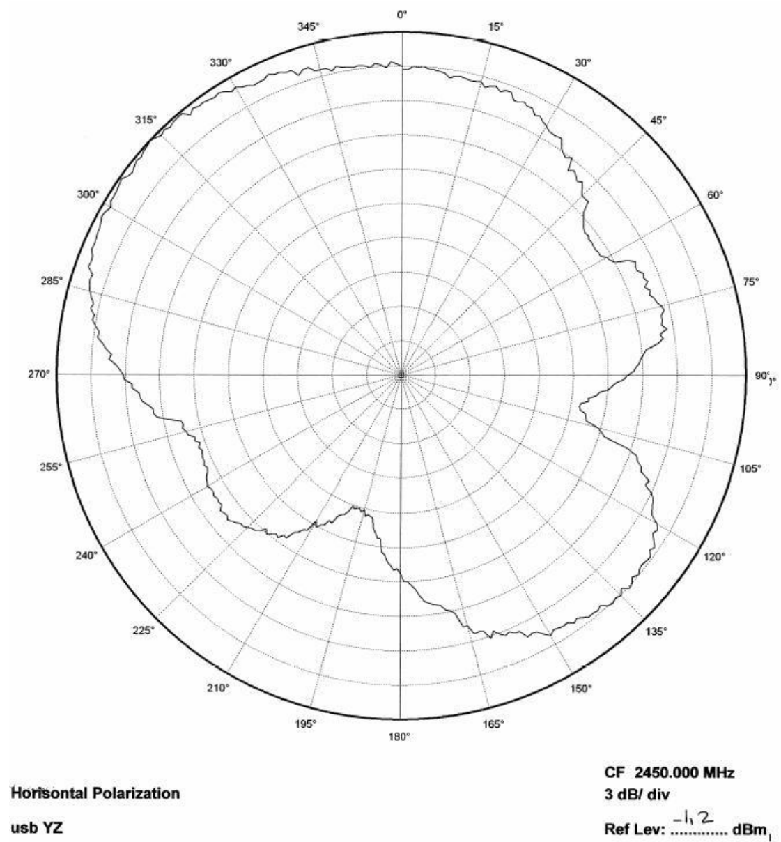
Figure 12: D63Beacon YZ Plane
