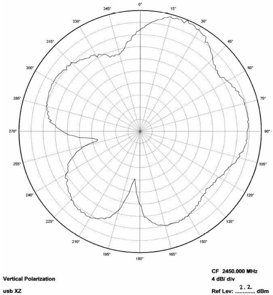
Figure 9: D63Beacon XZ Plane
