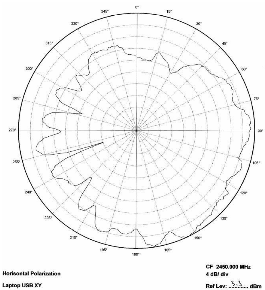
Figure 14: D63Beacon in Laptop XY
