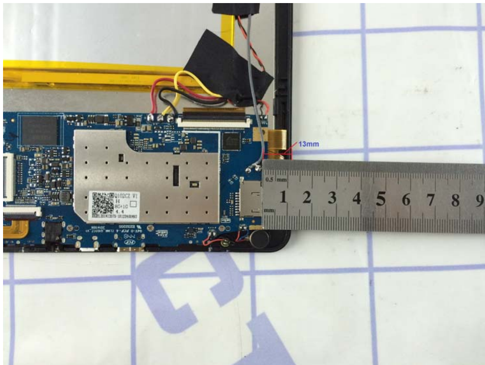
Antenna separation distance view-1
