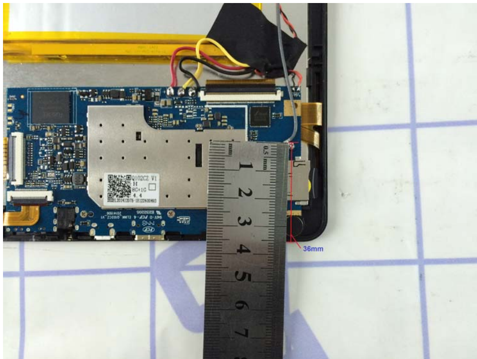
Antenna separation distance view-2
