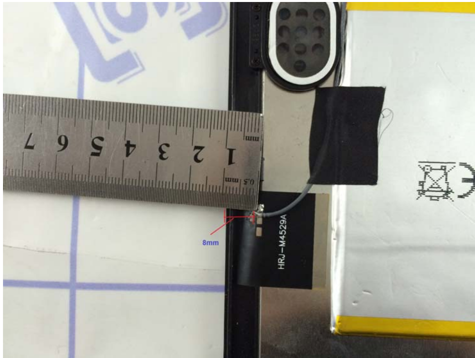
Antenna separation distance view-5
