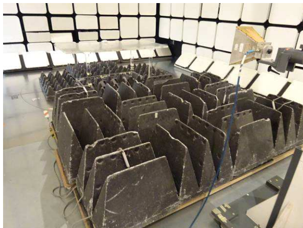
Radio-frequency radiated emissions (1 – 12.5 GHz)
