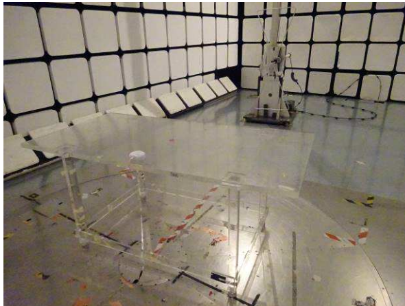
Unwanted emissions into Restricted Frequency Bands (30 MHz -1 GHz), Unwanted emissions into non-Restricted Frequency Bands (30 MHz -1 GHz) and Radio-frequency radiated emissions (30 MHz – 1 GHz)
