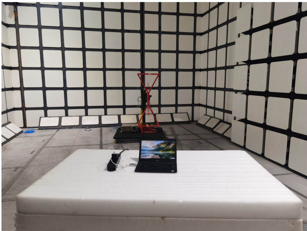
Radiated Emissions View (Below 1GHz TX)
