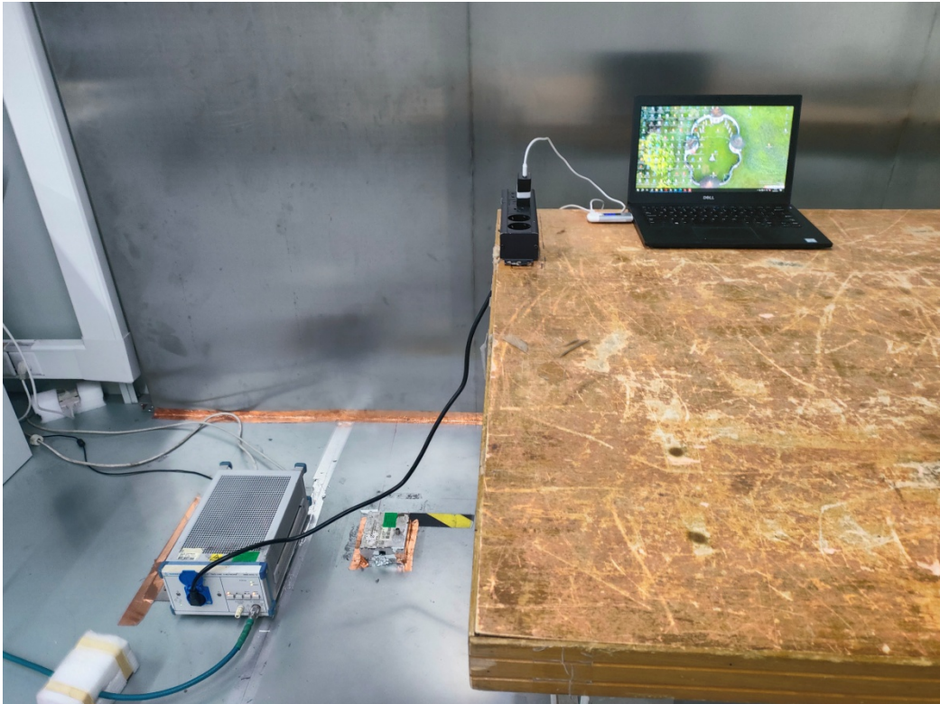
Conducted Emissions -TX Front View
