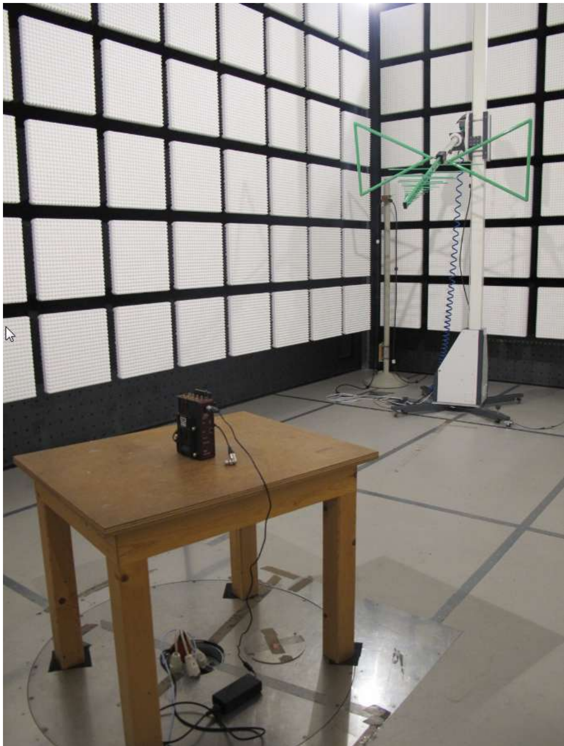
Photograph 2: Radiated emissions test set up, 30 – 1000 MHz
