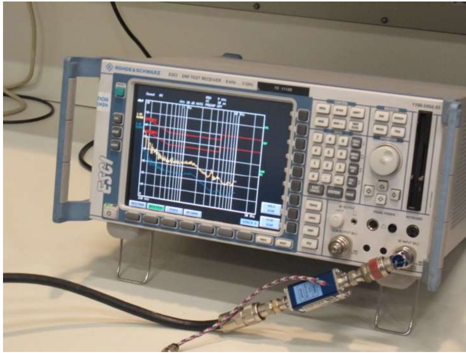
Photograph 5: EMI Test Receiver for Conducted AC power emission
