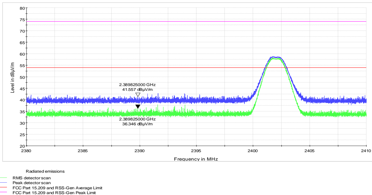
Figure 8.6-11: Radiated spurious emissions within restricted bands, lower band edge
