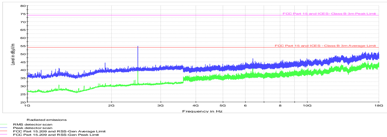
Figure 8.6-18: Radiated spurious emissions above 1 GHz, high channel
