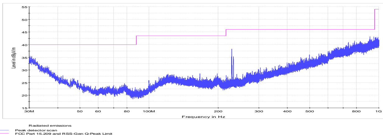
Figure 8.6-14: Radiated spurious emissions below 1 GHz, mid channel
