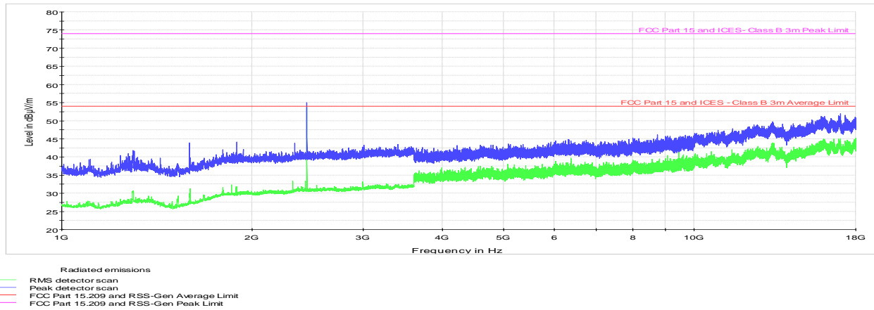
Figure 8.6-17: Radiated spurious emissions above 1 GHz, mid channel
