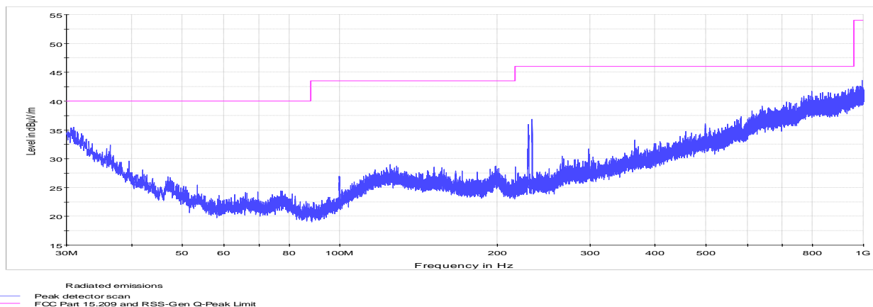
Figure 8.6-13: Radiated spurious emissions below 1 GHz, low channel
