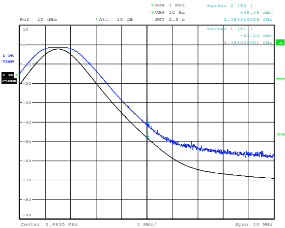
Figure 8.6-8: Conducted spurious emissions within restricted bands, high channel
