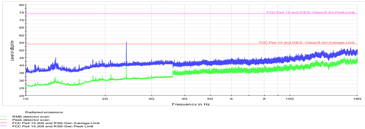
Figure 8.6-16: Radiated spurious emissions above 1 GHz, low channel
