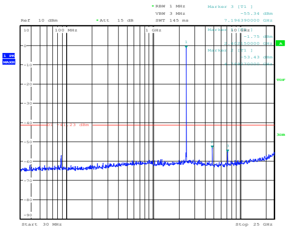
Figure 8.6-4: Conducted spurious emissions at the lower band edge
