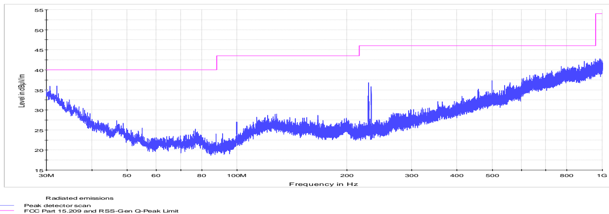
Figure 8.6-15: Radiated spurious emissions below 1 GHz, high channel
