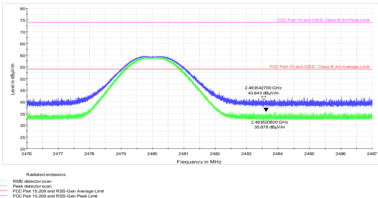
Figure 8.6-12: Radiated spurious emissions within restricted bands, upper band edge
