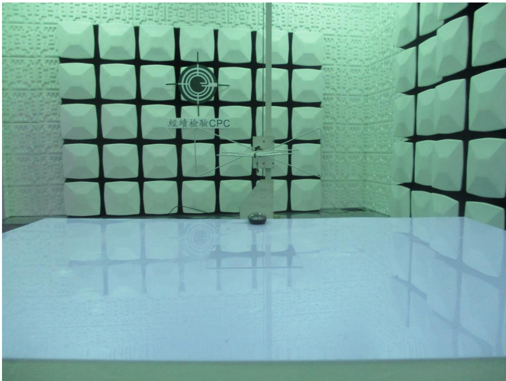
Setup Photo FCC ID: 2ACKHXW6906
