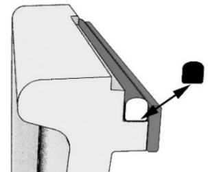
Be careful not to twist the seals when installing
