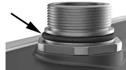
Be careful not to twist the seals when installing
