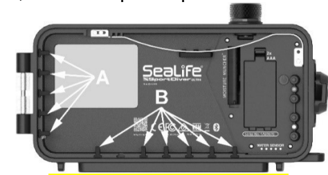
Pre-installed rubber grip tabs
