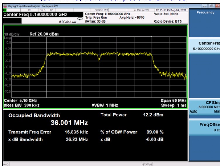
(802.11n40) Bandwidth plot on channel 38
