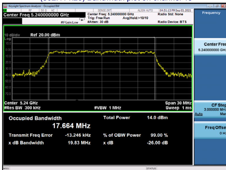
(802.11 n20) Bandwidth plot on channel 48
