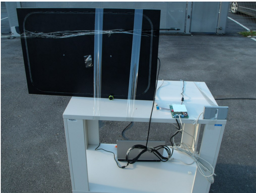
Figure 8: Radiated emission tests - OATS
