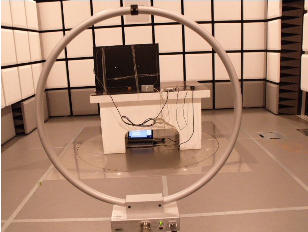
Figure 3: Radiated emission test from 9 kHz to 30 MHz
