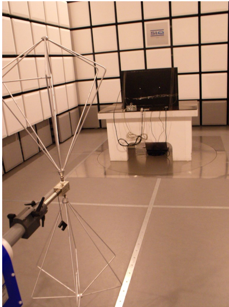
Figure 5: Radiated emission test from 30 MHz to 200 MHz
