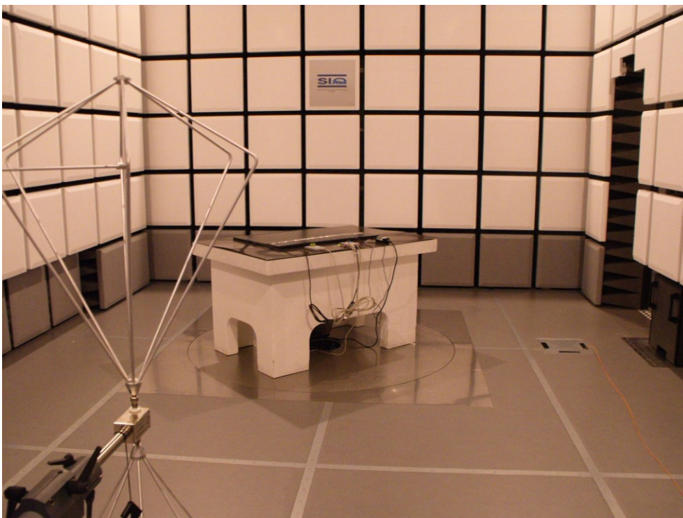
Figure 4: Radiated emission test from 30 MHz to 200 MHz
