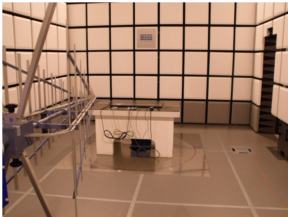
Figure 6: Radiated emission test from 200 MHz to 1 GHz
