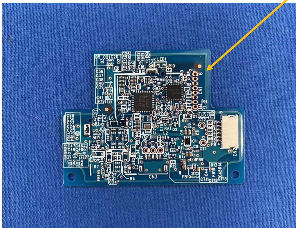
Component side wo shield
