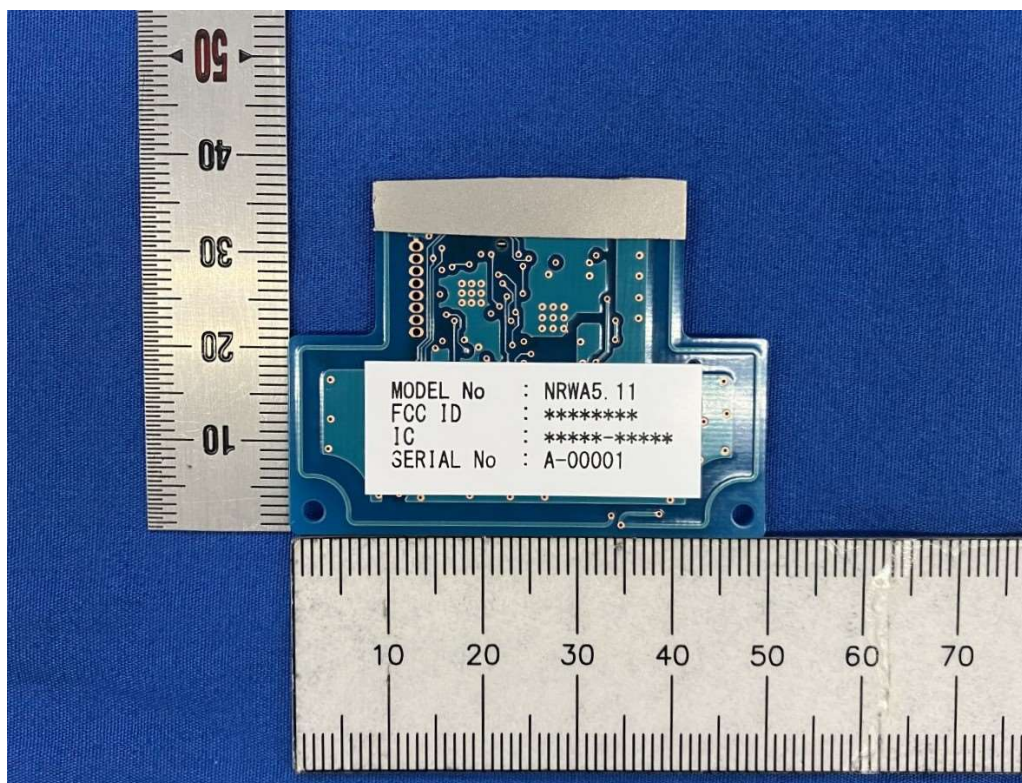
Rear side
