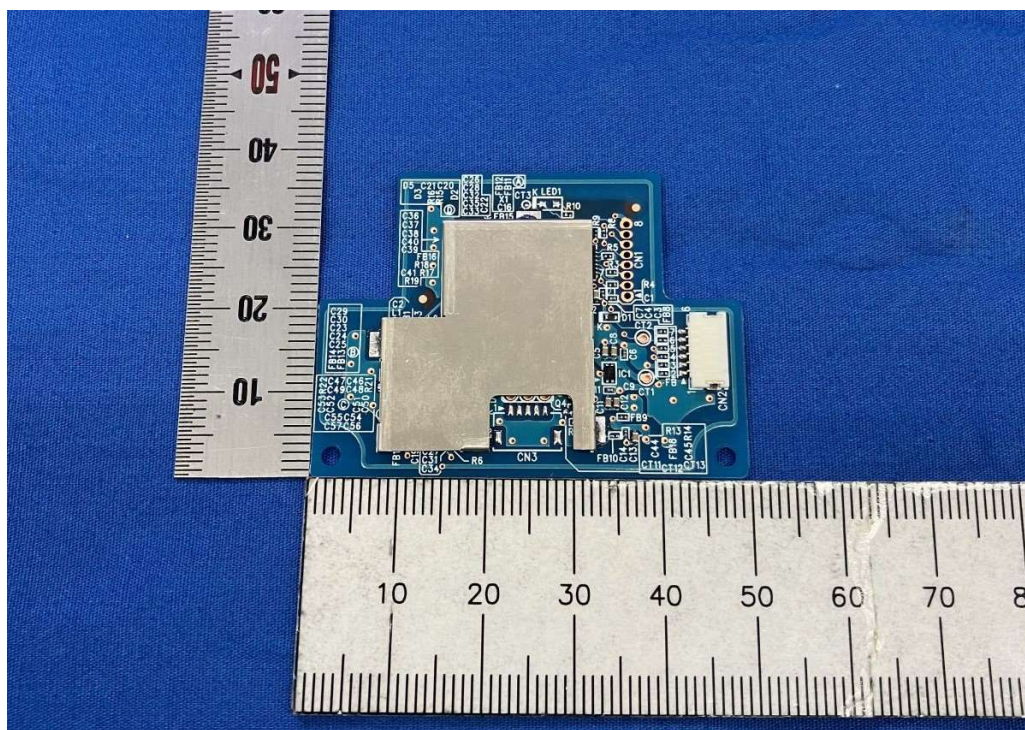
Component side
